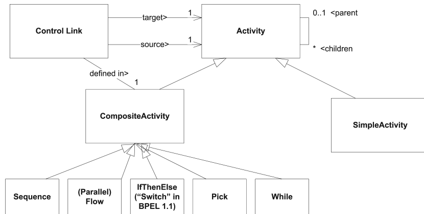
Fig. 2. Relevant fragment of the BPEL meta-model
