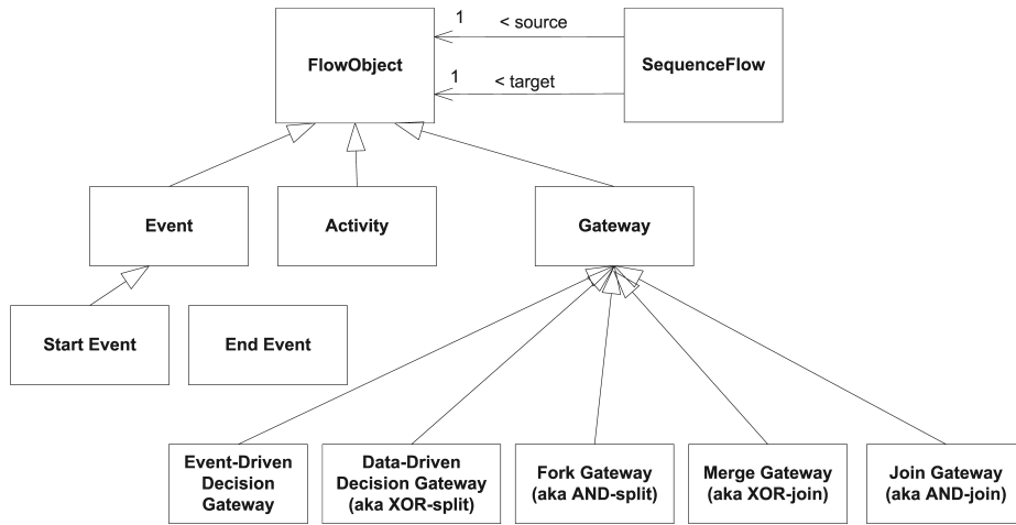
Fig. 1. Relevant fragment of the BPMN meta-model
